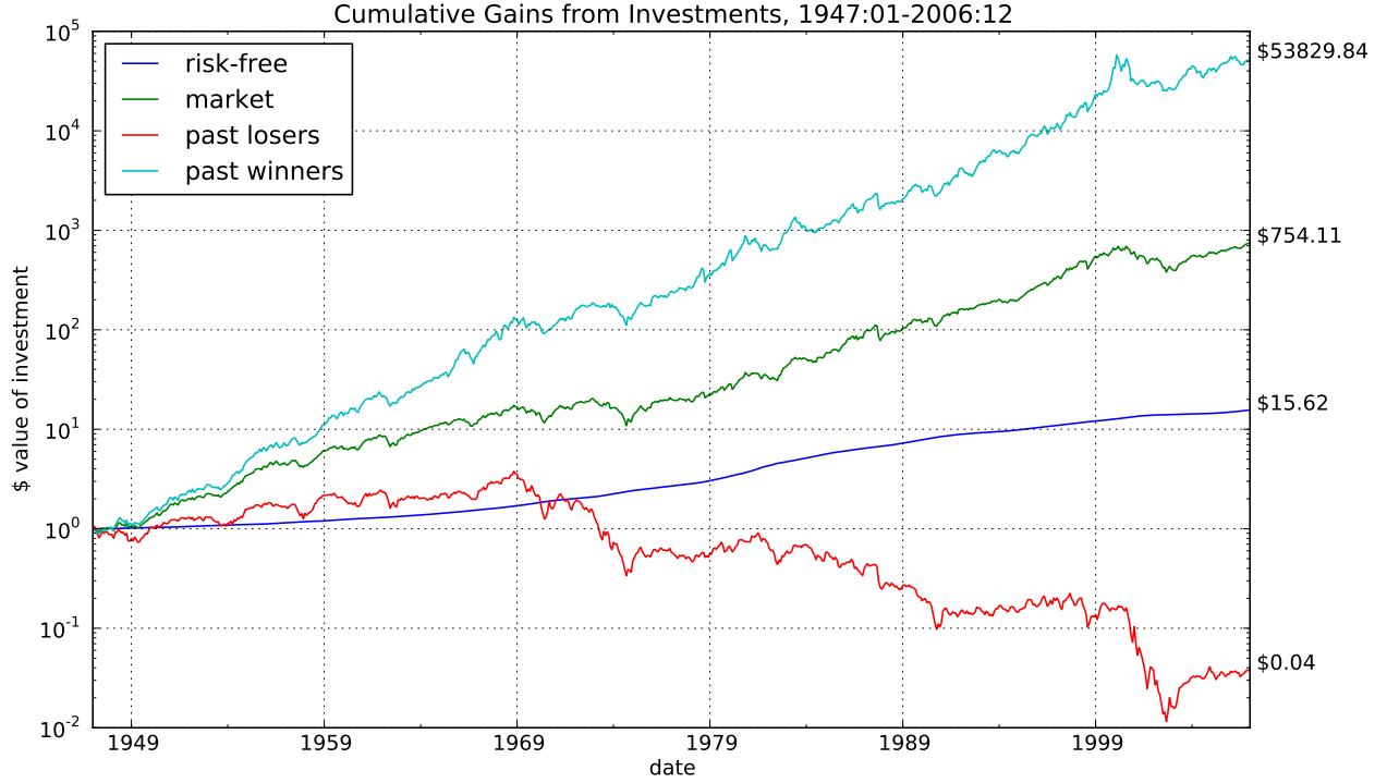
Figure 1: Momentum Components, 1947-2006
