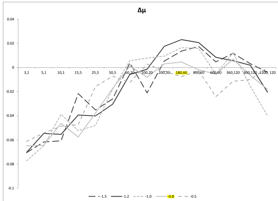
Fig. 3. Stopping premium, (\Delta_\mu) , from short-term (3,1) stop-loss strategies to longer-term (1200,120) stop-loss strategies with exit thresholds, (\gamma) , of 1.5, 1.2, 1, 0.8, and 0.5 standard deviations from the mean with a 0 standard deviation re-entry threshold, (\delta)
